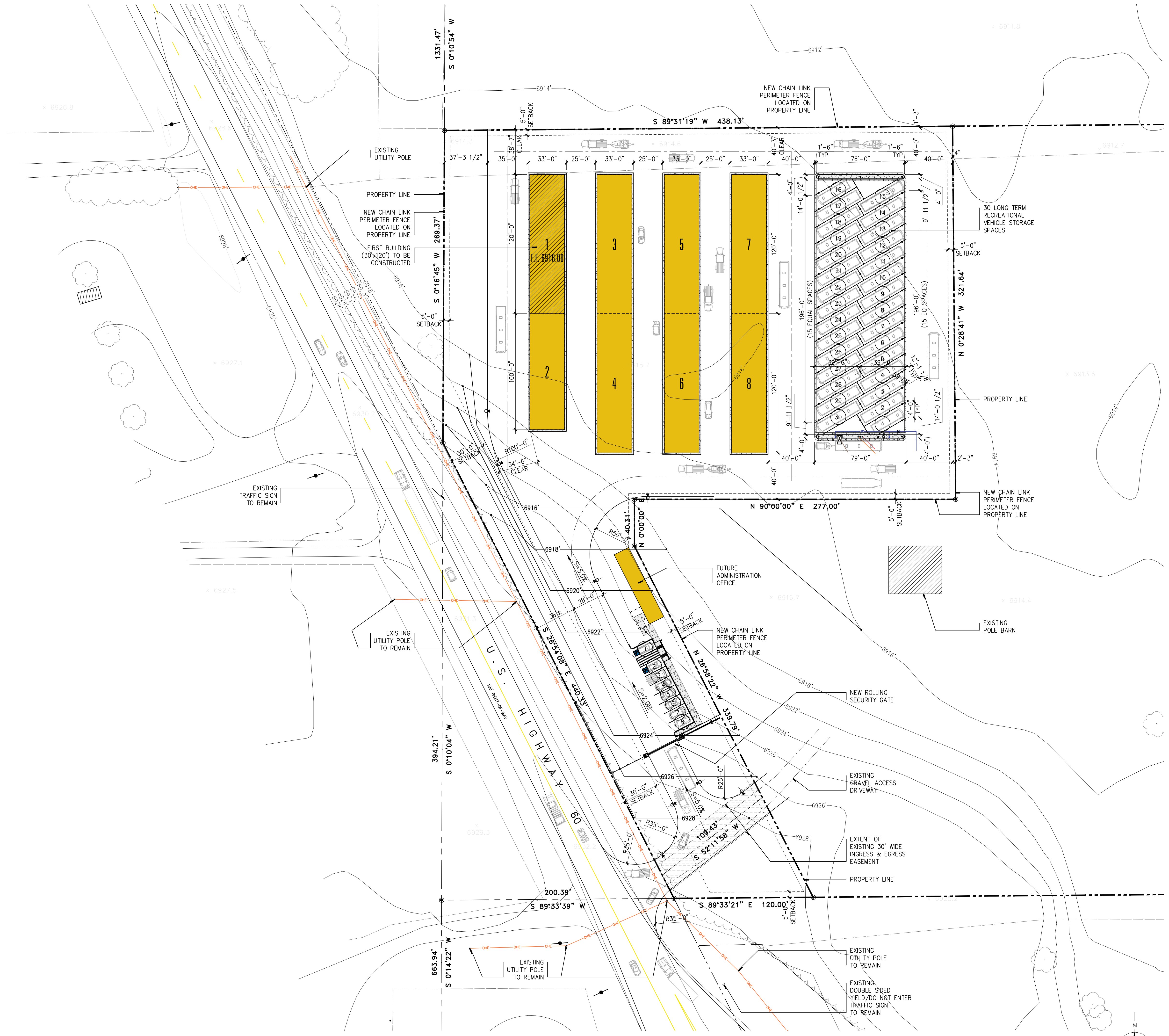
SITE PLAN
