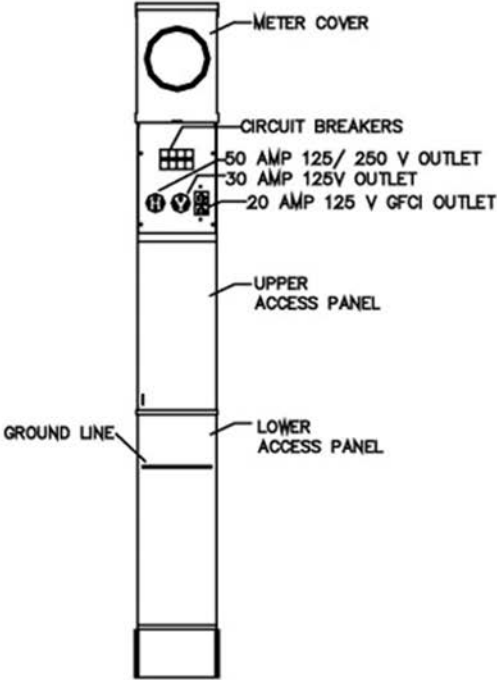
FRONT VIEW ROTATING BREAKER PANEL COVER REMOVED
